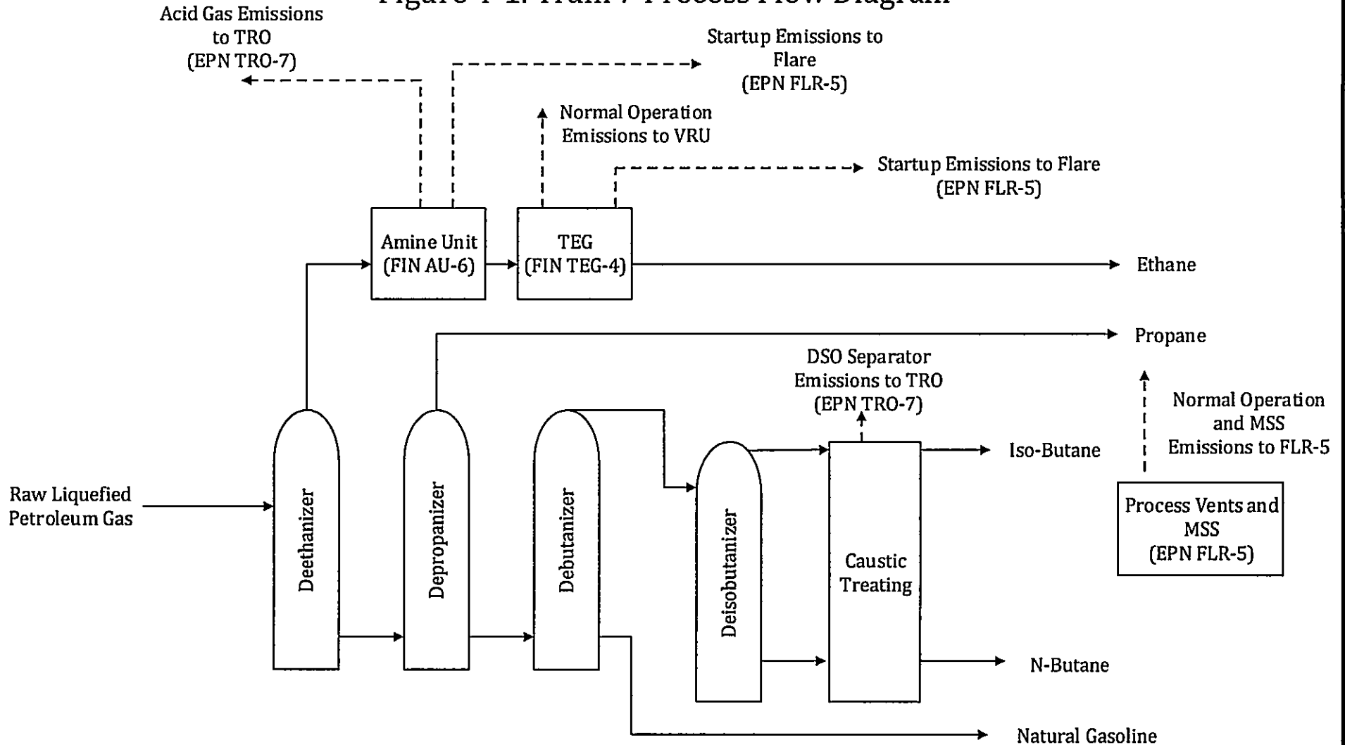
Figure 4-1. Train 7 Process Flow Diagram
